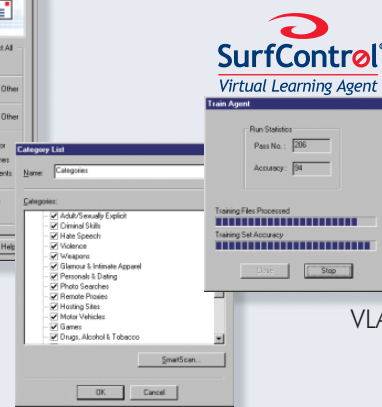
URL Categories
