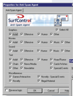
Anti-Spam Agent™
